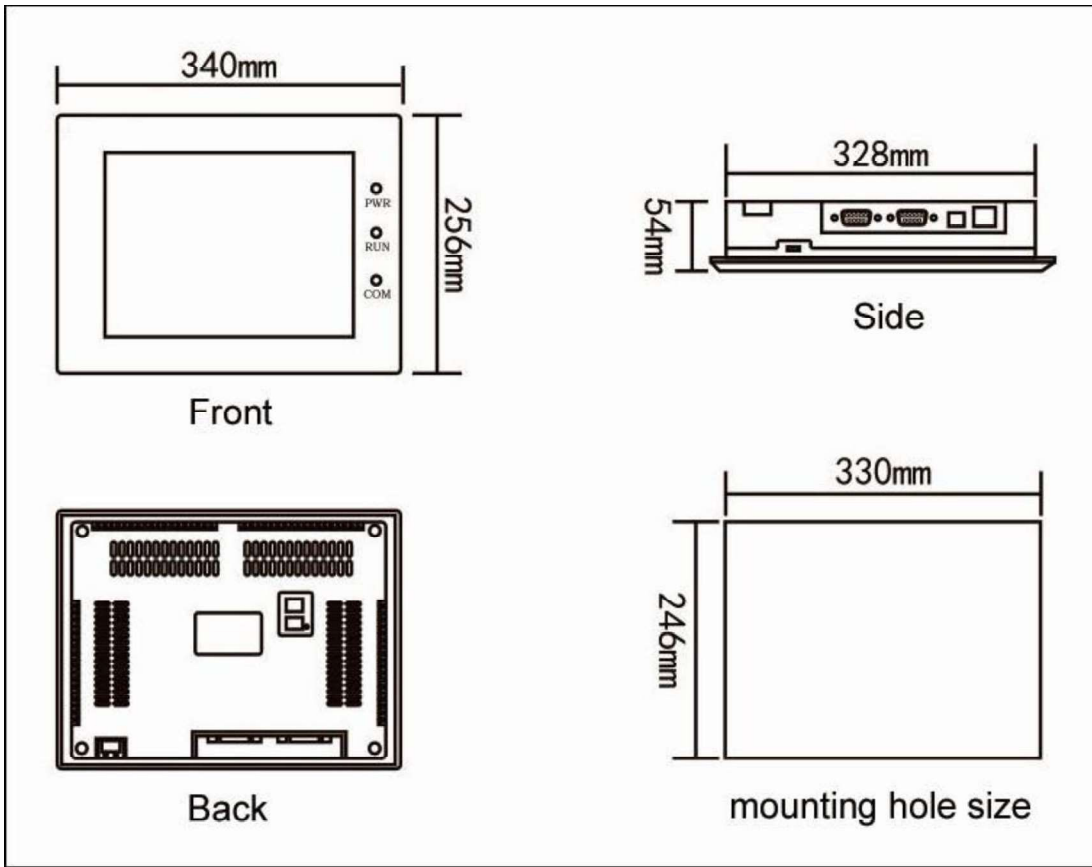
Figure 1-8 HT8C21T mounting dimension
