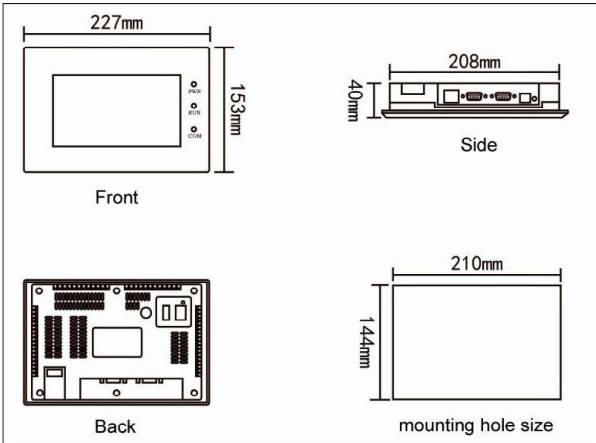
Figure 1-5 HT8701 mounting dimension
