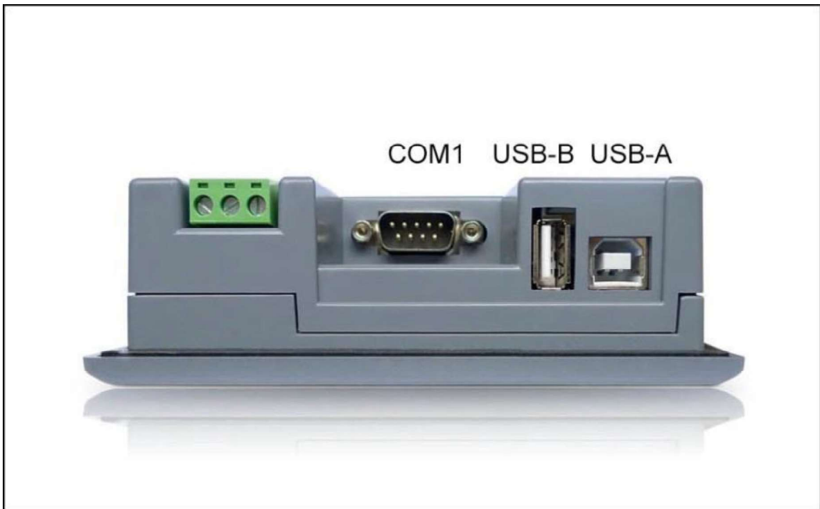
Figure 1-13 Side panels of HT (single serial)
