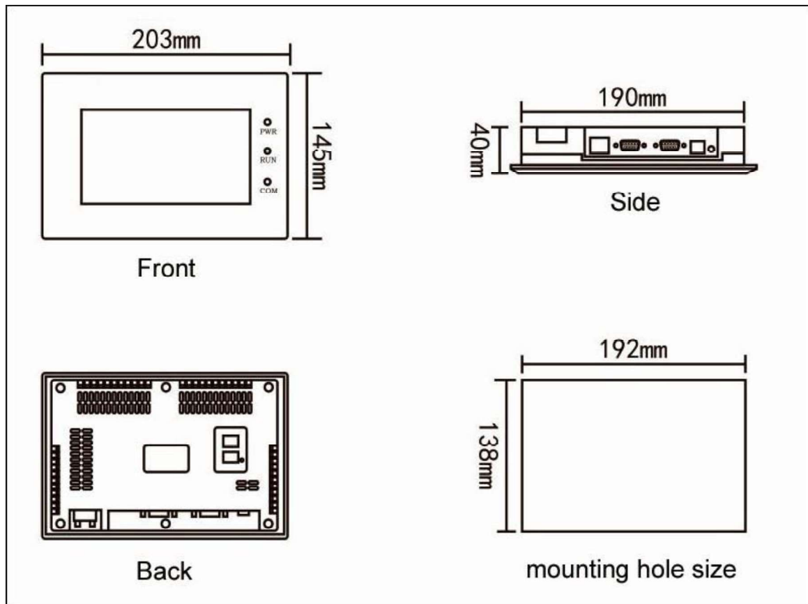
Figure 1-6 HT8721T mounting dimension
