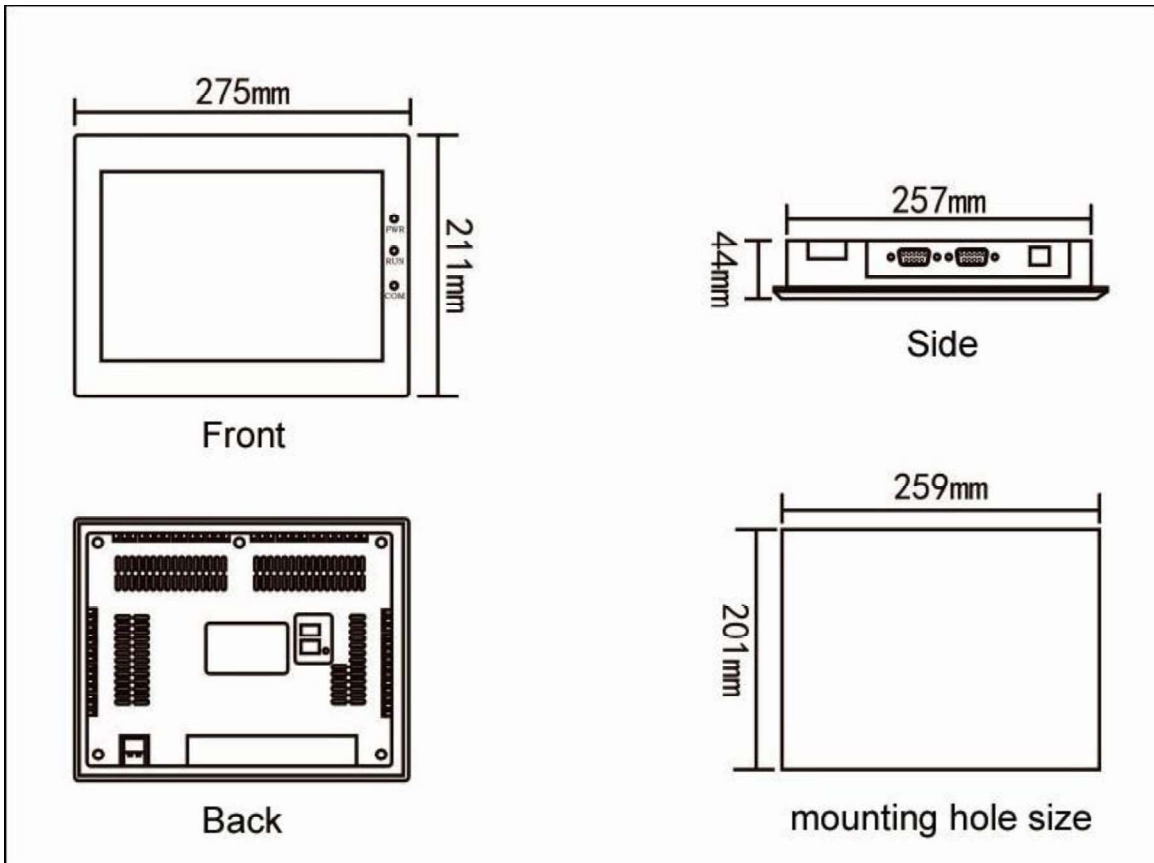
Figure 1-7 HT8A01T / HT8A01T E mounting dimension
