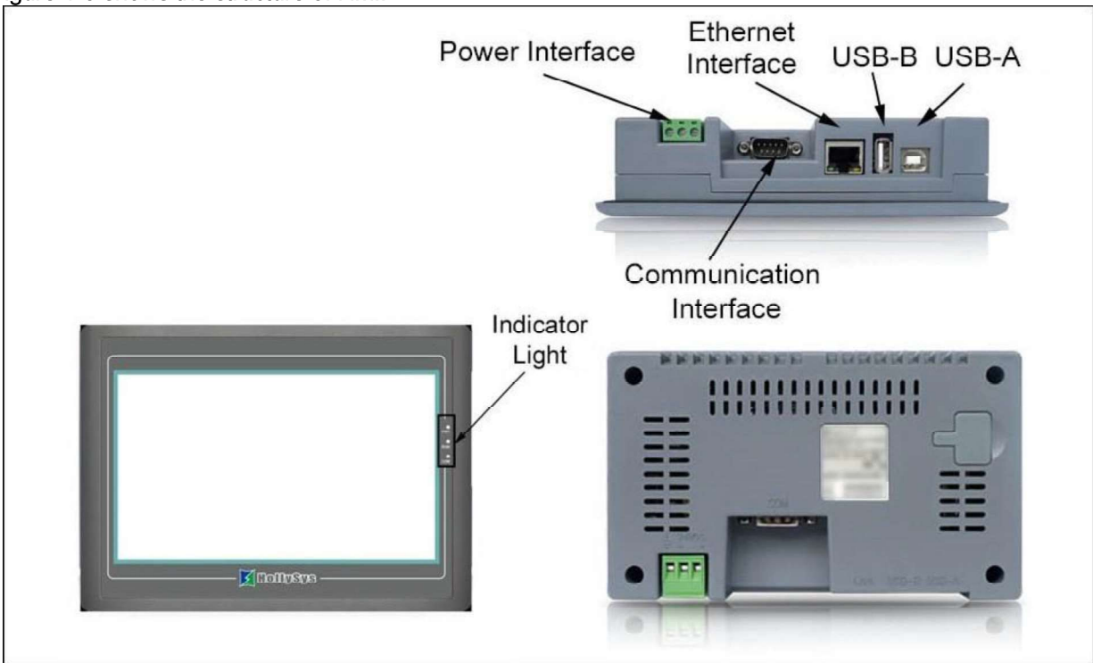
Figure 1-9 Structure
