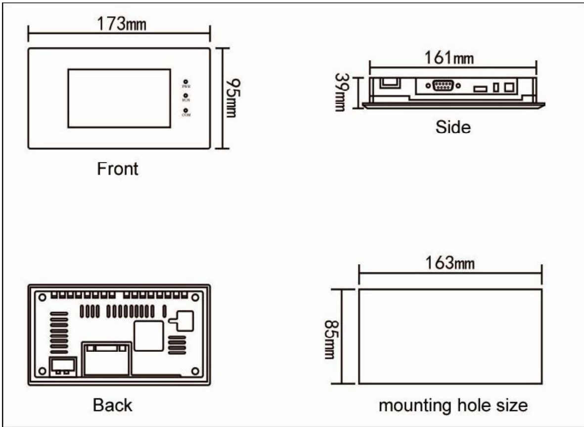
Figure 1-3 HT8421T mounting dimension
