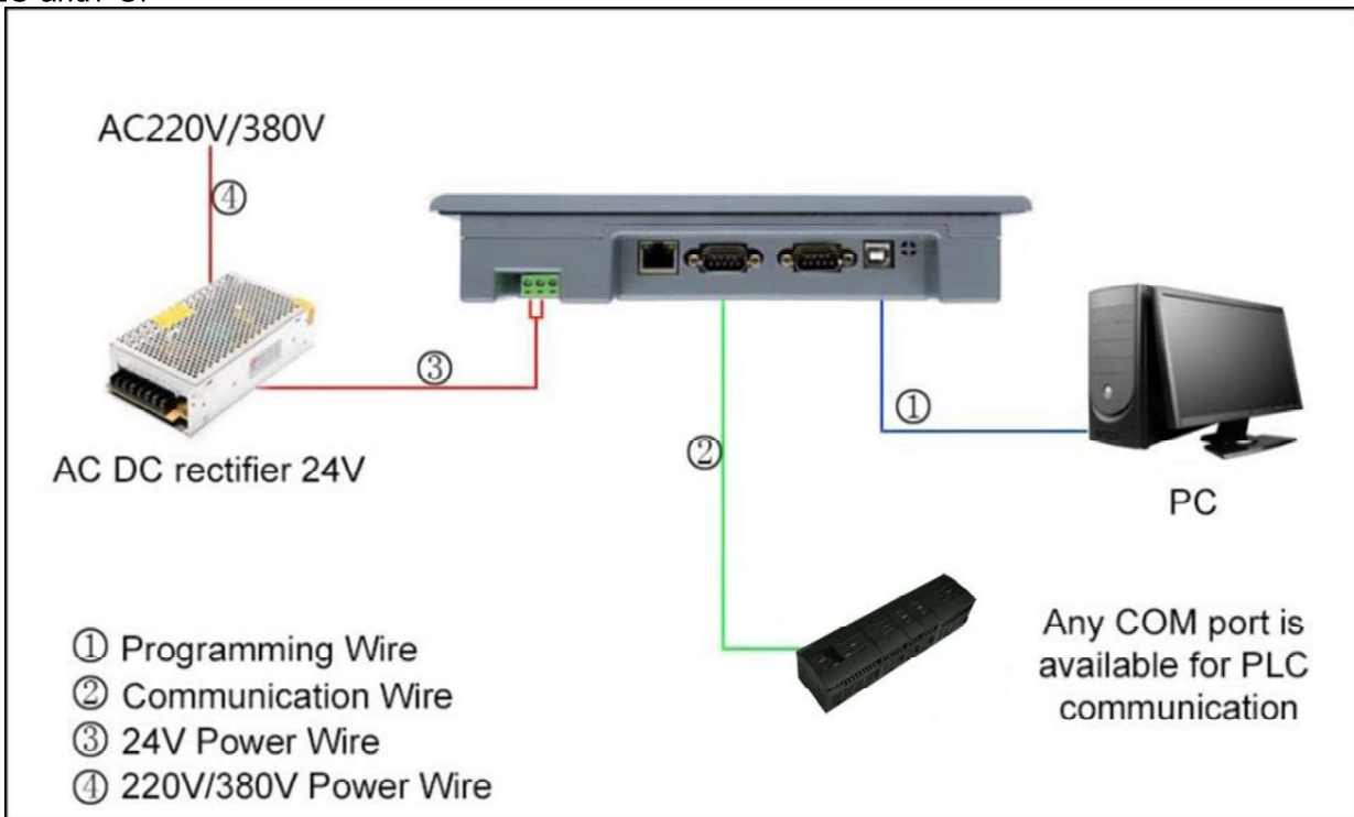
Figure 1-16 Connection diagram of HT series HMI
